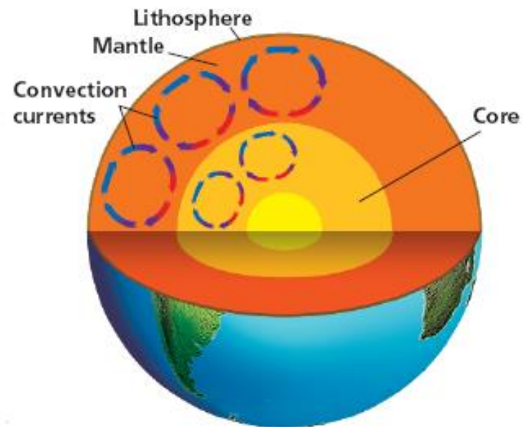
Mantle Convection
