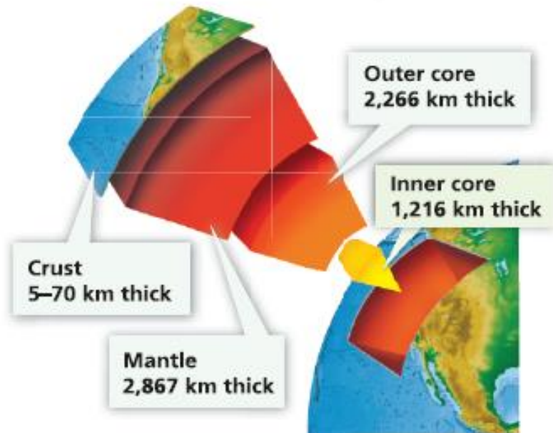
Earth's Layers
